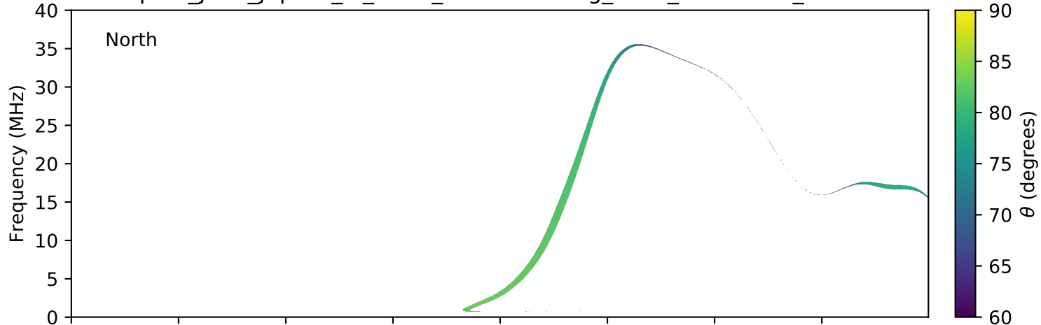
expres_juno_jupiter_io_isaac_lossc-wid1deg_3kev_20171001_v01.cdf
