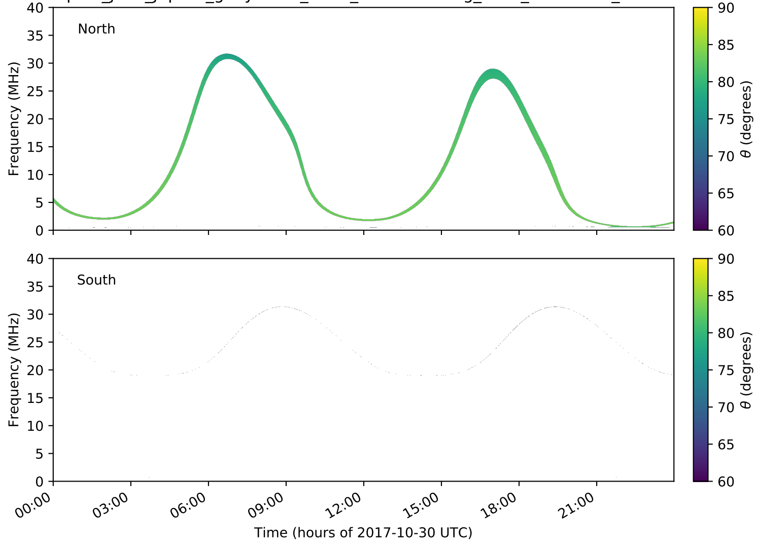
expres_juno_jupiter_ganymede_isaac_lossc-wid1deg_3kev_20171030_v01.cdf
