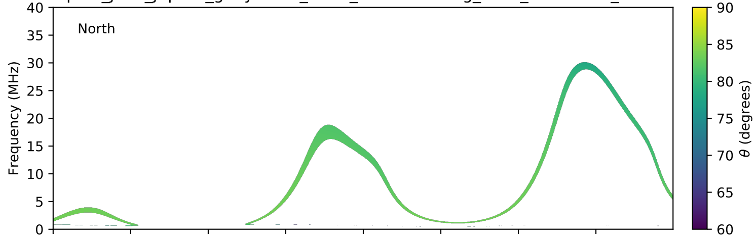
expres_juno_jupiter_ganymede_isaac_lossc-wid1deg_3kev_20171029_v01.cdf
