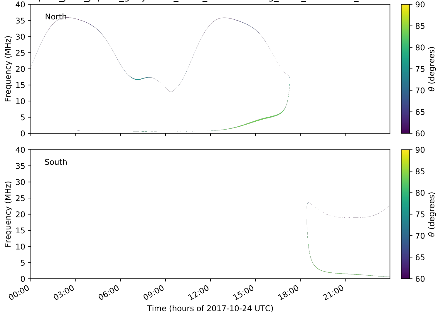
expres_juno_jupiter_ganymede_isaac_lossc-wid1deg_3kev_20171024_v01.cdf
