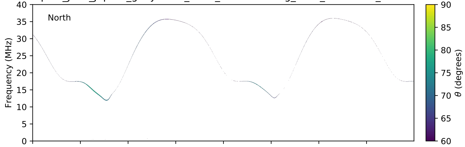
expres_juno_jupiter_ganymede_isaac_lossc-wid1deg_3kev_20171022_v01.cdf
