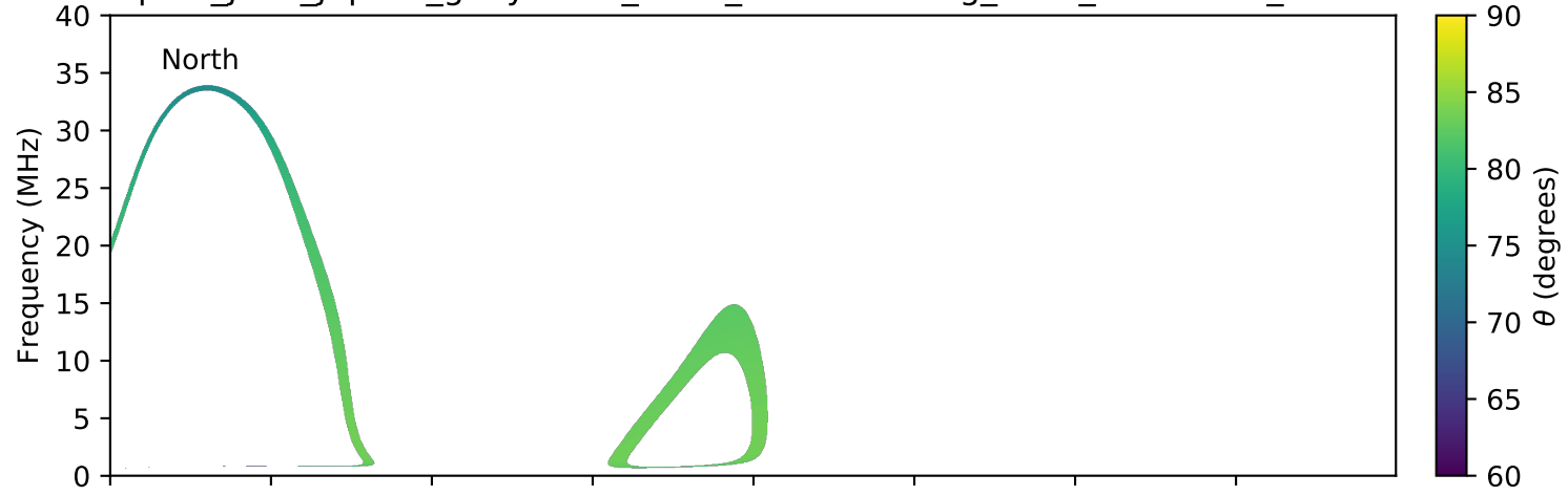
expres_juno_jupiter_ganymede_isaac_lossc-wid1deg_3kev_20171017_v01.cdf
