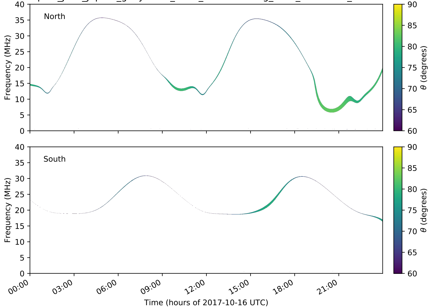
expres_juno_jupiter_ganymede_isaac_lossc-wid1deg_3kev_20171016_v01.cdf
