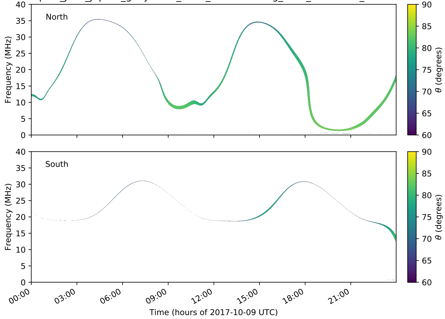
expres_juno_jupiter_ganymede_isaac_lossc-wid1deg_3kev_20171009_v01.cdf
