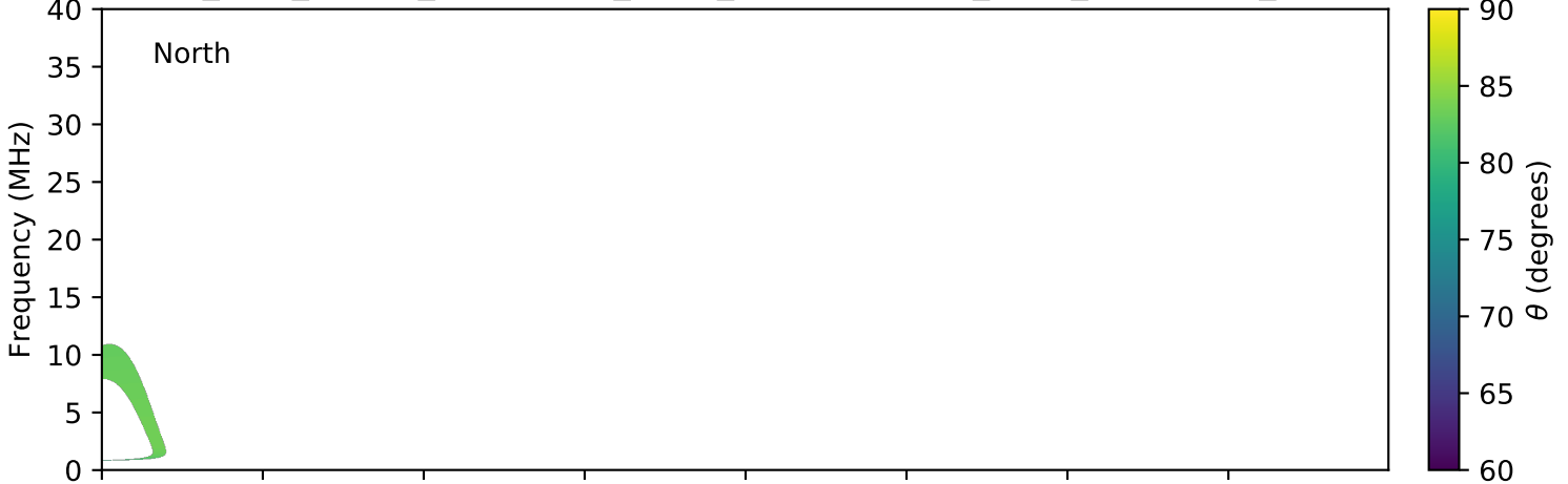
expres_juno_jupiter_ganymede_isaac_lossc-wid1deg_3kev_20171003_v01.cdf
