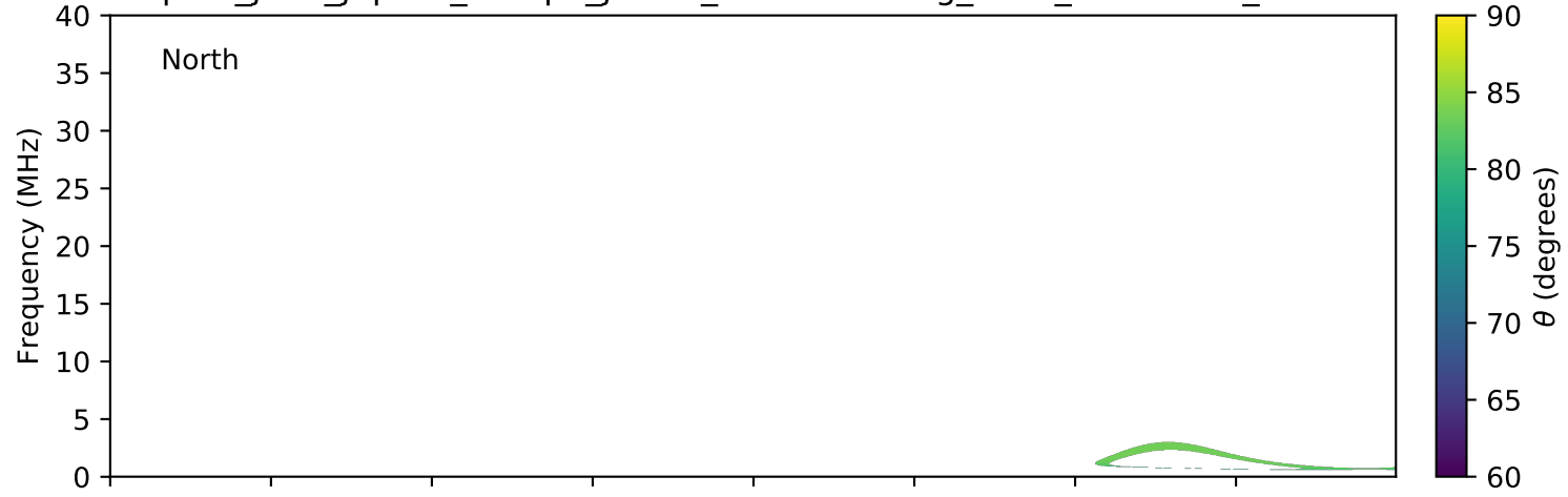
expres_juno_jupiter_europa_jrm09_lossc-wid1deg_3kev_20171027_v01.cdf
