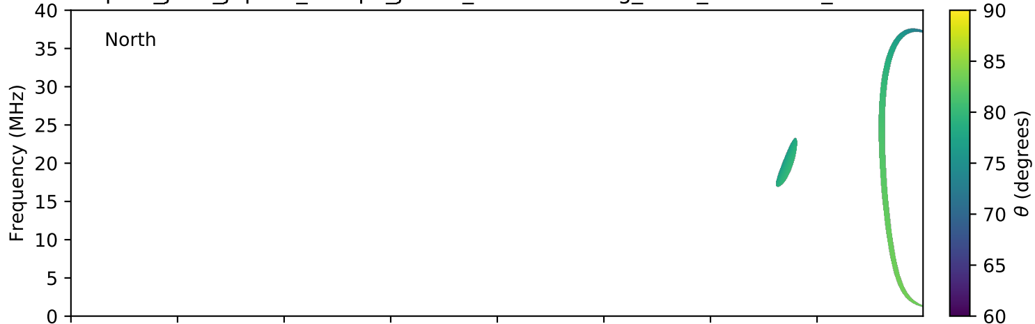
expres_juno_jupiter_europa_jrm09_lossc-wid1deg_3kev_20171023_v01.cdf
