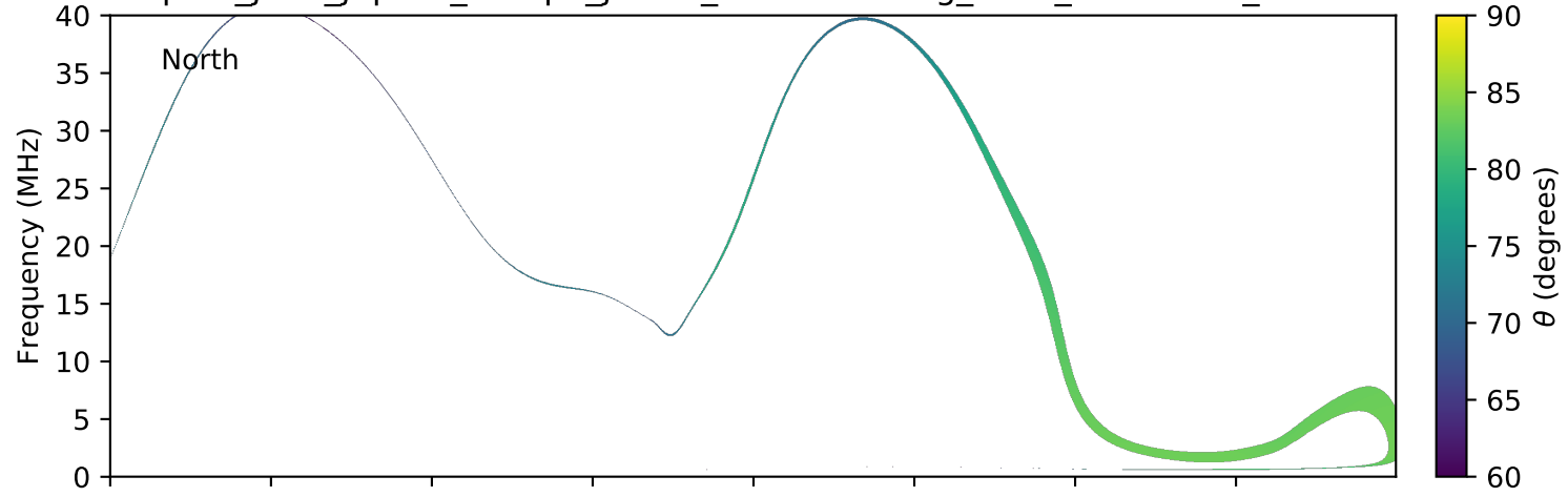
expres_juno_jupiter_europa_jrm09_lossc-wid1deg_3kev_20171014_v01.cdf
