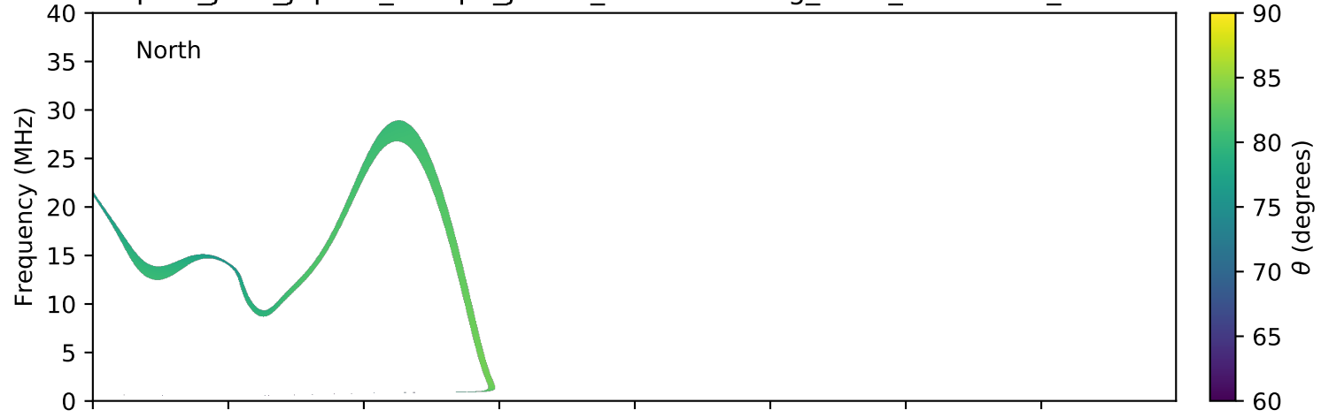
expres_juno_jupiter_europa_jrm09_lossc-wid1deg_3kev_20171011_v01.cdf
