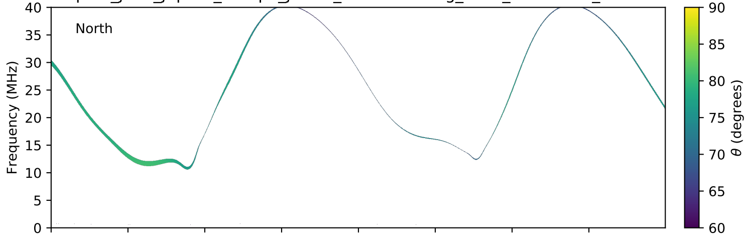
expres_juno_jupiter_europa_jrm09_lossc-wid1deg_3kev_20171010_v01.cdf
