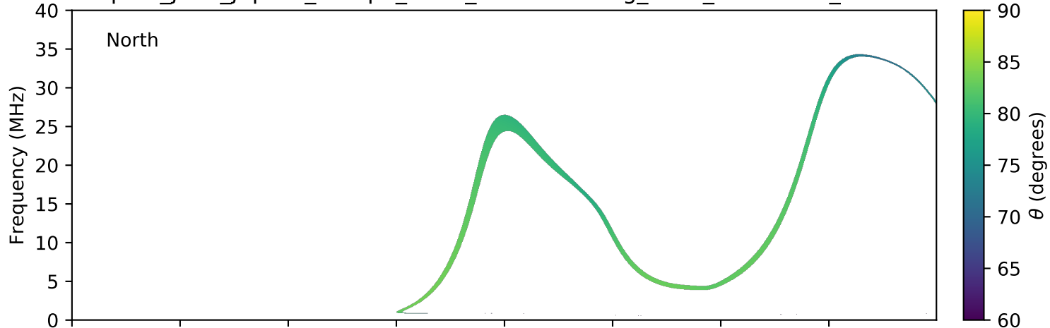
expres_juno_jupiter_europa_isaac_lossc-wid1deg_3kev_20171031_v01.cdf
