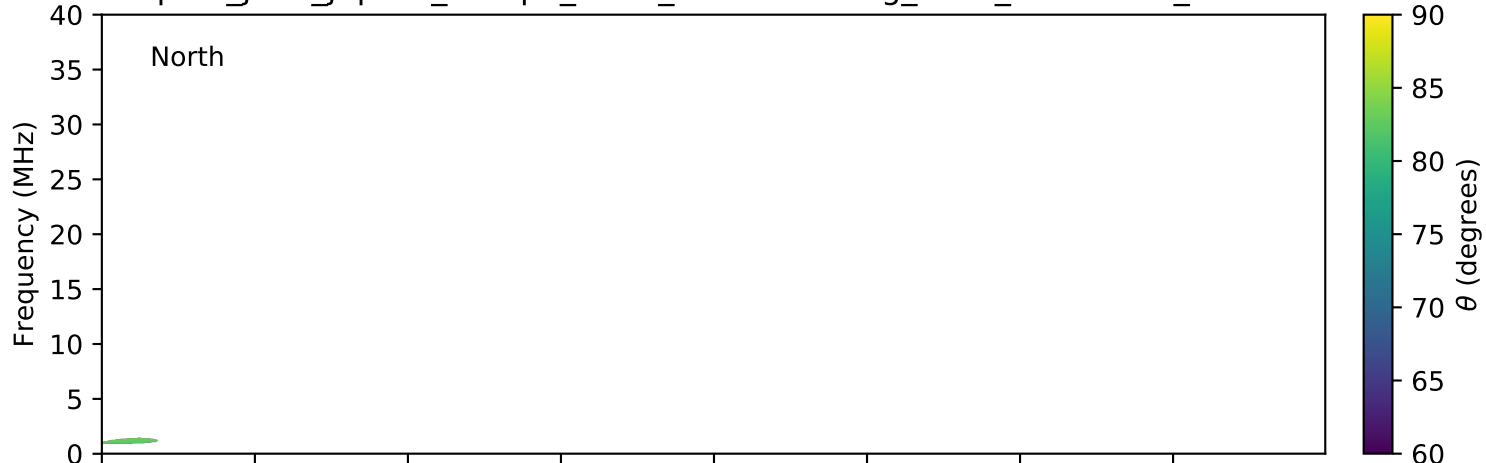
expres_juno_jupiter_europa_isaac_lossc-wid1deg_3kev_20171029_v01.cdf
