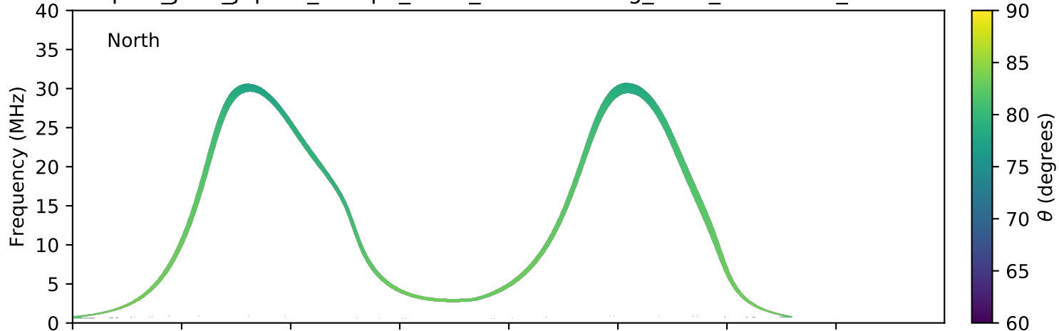
expres_juno_jupiter_europa_isaac_lossc-wid1deg_3kev_20171028_v01.cdf
