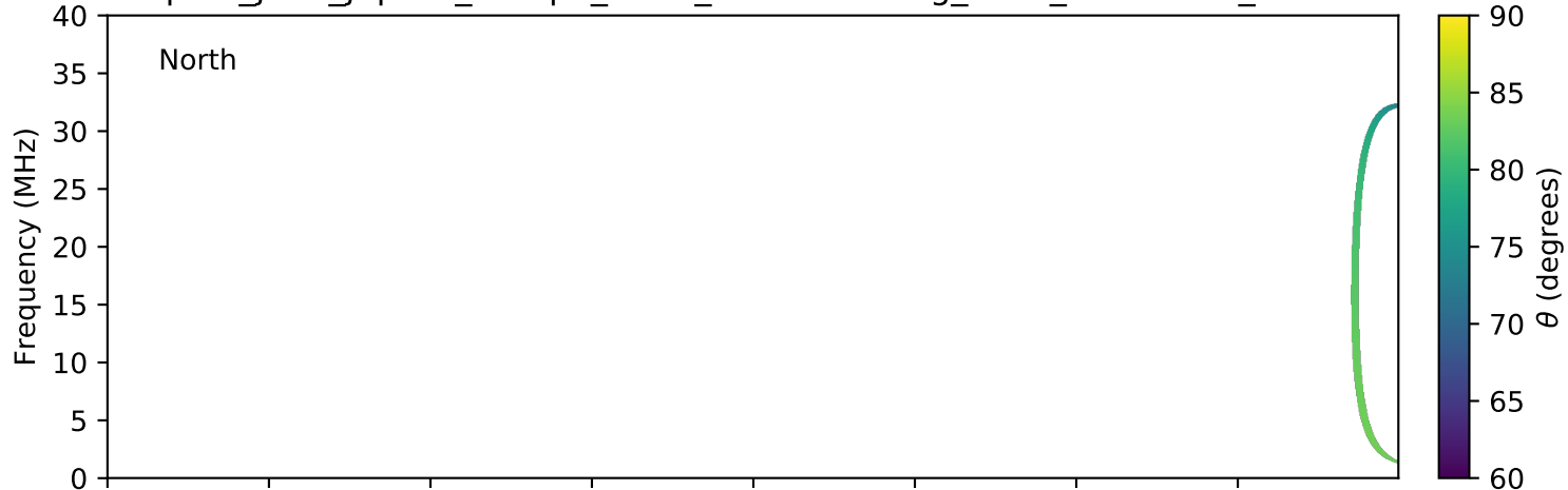
expres_juno_jupiter_europa_isaac_lossc-wid1deg_3kev_20171023_v01.cdf
