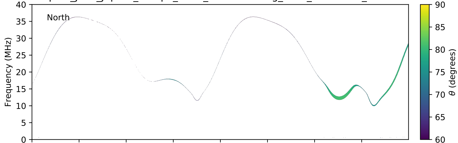
expres_juno_jupiter_europa_isaac_lossc-wid1deg_3kev_20171021_v01.cdf
