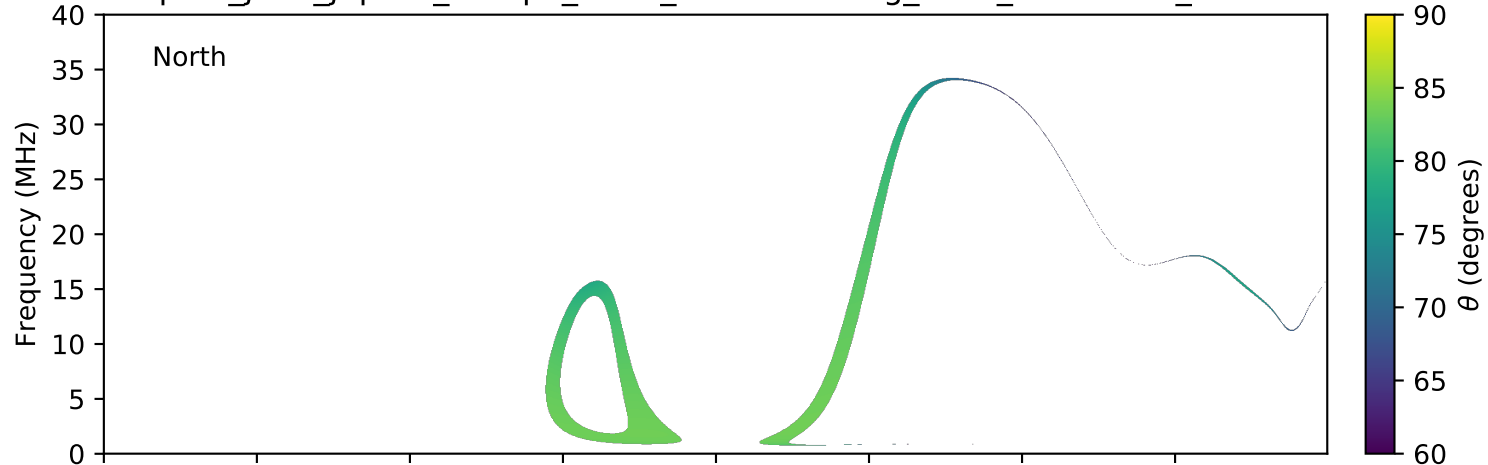
expres_juno_jupiter_europa_isaac_lossc-wid1deg_3kev_20171020_v01.cdf
