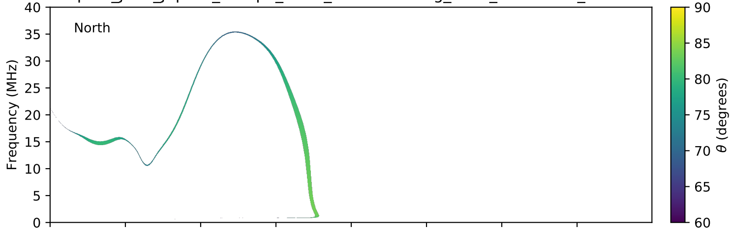
expres_juno_jupiter_europa_isaac_lossc-wid1deg_3kev_20171018_v01.cdf
