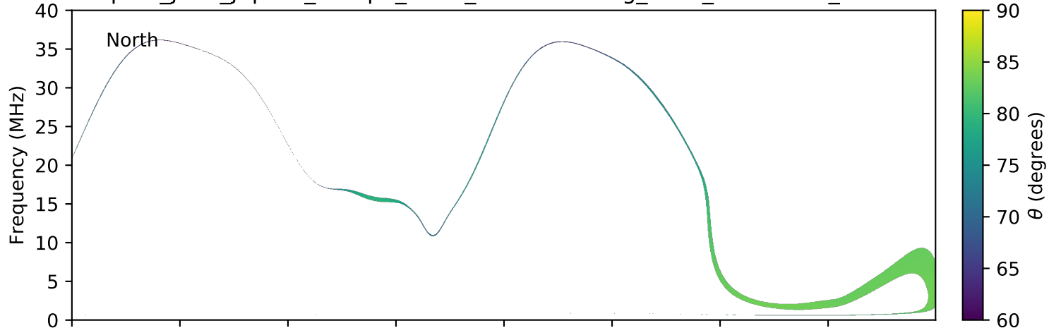
expres_juno_jupiter_europa_isaac_lossc-wid1deg_3kev_20171014_v01.cdf
