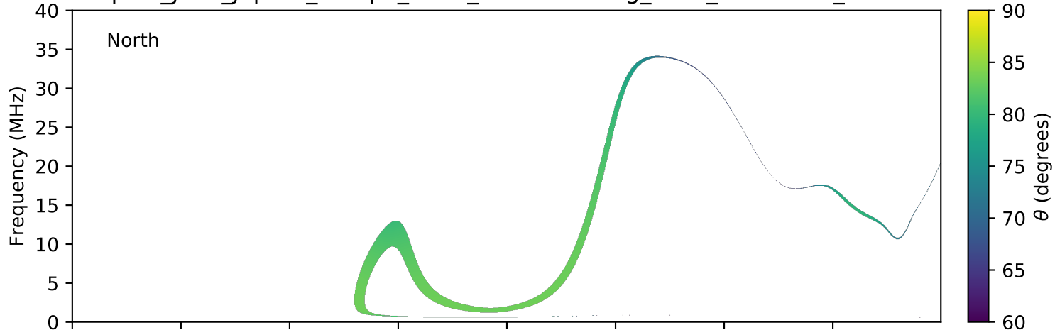
expres_juno_jupiter_europa_isaac_lossc-wid1deg_3kev_20171013_v01.cdf
