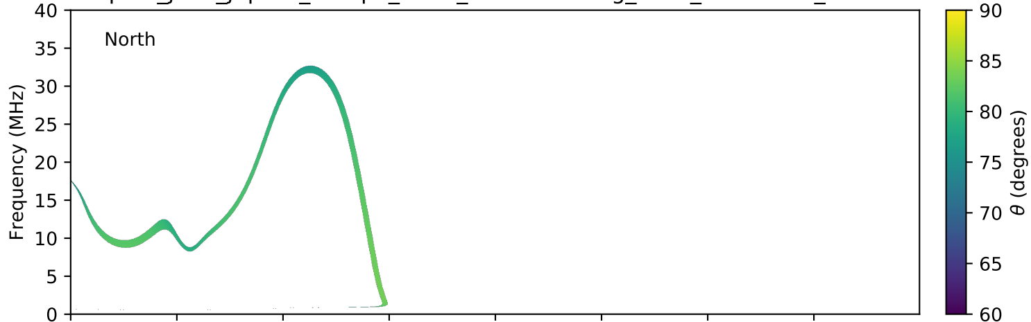
expres_juno_jupiter_europa_isaac_lossc-wid1deg_3kev_20171011_v01.cdf
