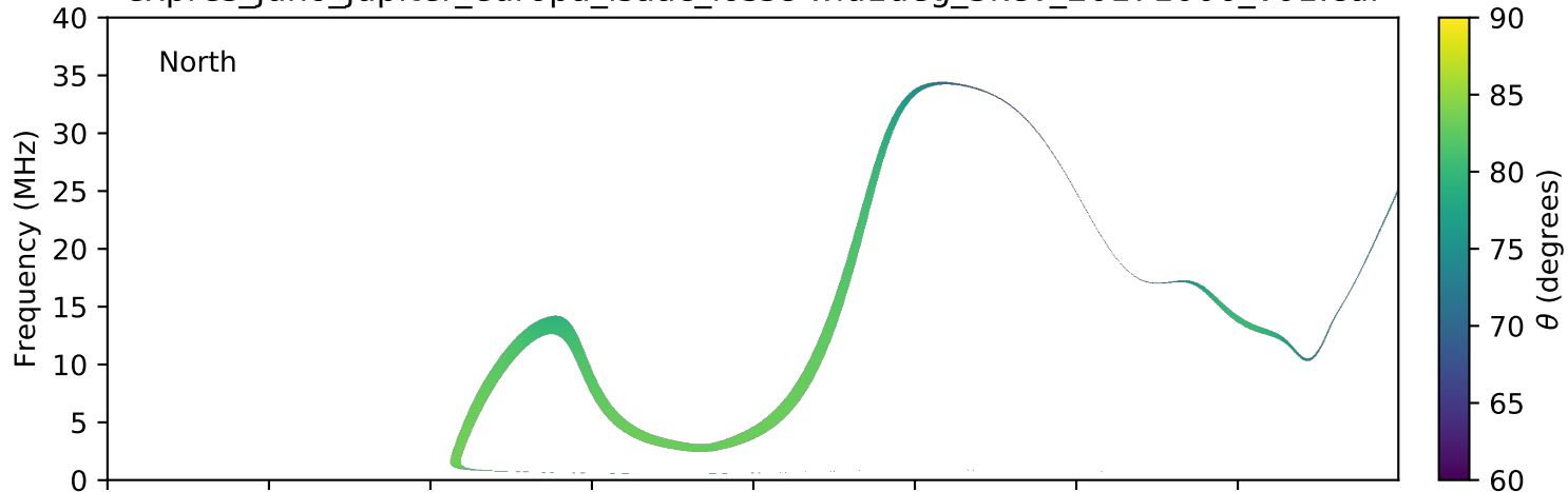
expres_juno_jupiter_europa_isaac_lossc-wid1deg_3kev_20171006_v01.cdf
