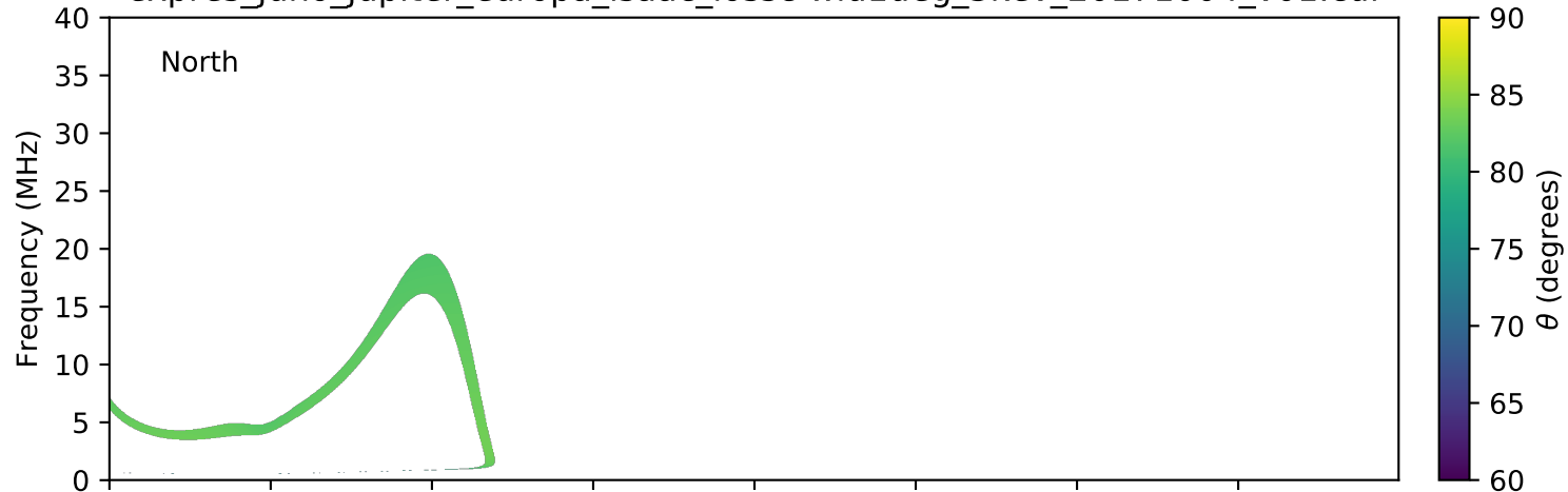
expres_juno_jupiter_europa_isaac_lossc-wid1deg_3kev_20171004_v01.cdf
