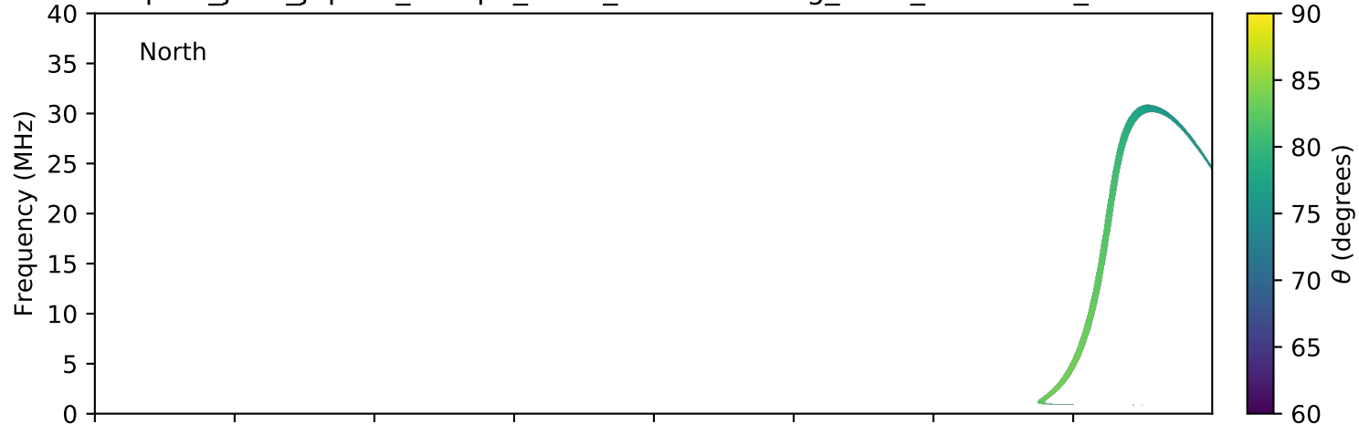
expres_juno_jupiter_europa_isaac_lossc-wid1deg_3kev_20171002_v01.cdf
