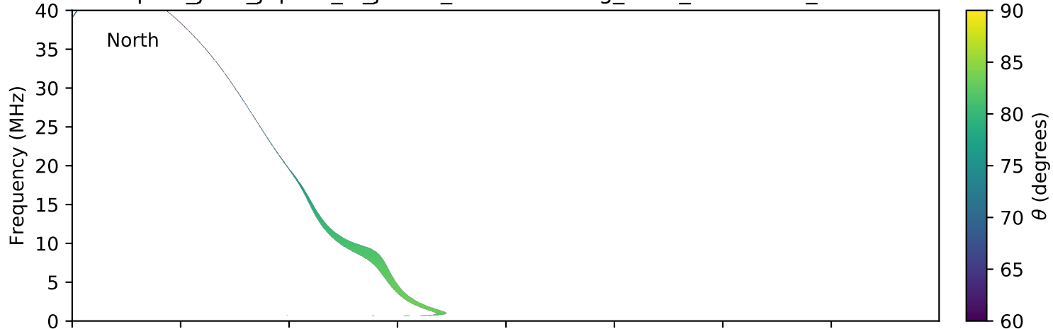
expres_juno_jupiter_io_jrm09_lossc-wid1deg_3kev_20170930_v01.cdf
