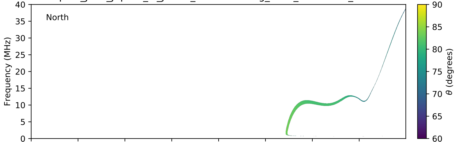
expres_juno_jupiter_io_jrm09_lossc-wid1deg_3kev_20170929_v01.cdf
