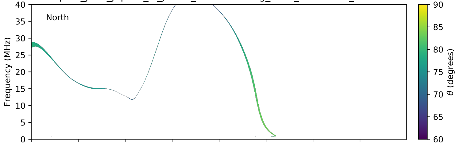
expres_juno_jupiter_io_jrm09_lossc-wid1deg_3kev_20170928_v01.cdf
