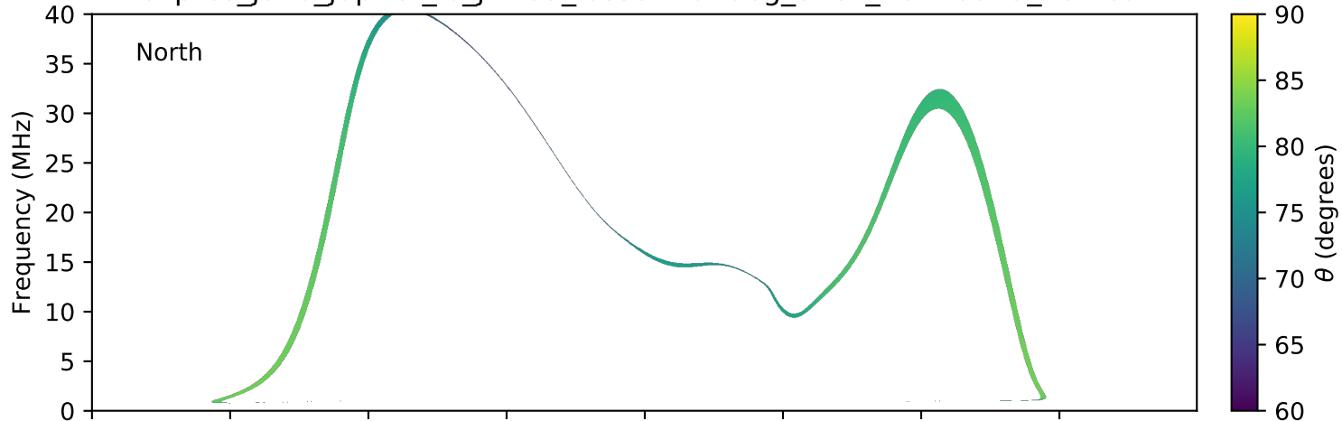
expres_juno_jupiter_io_jrm09_lossc-wid1deg_3kev_20170919_v01.cdf
