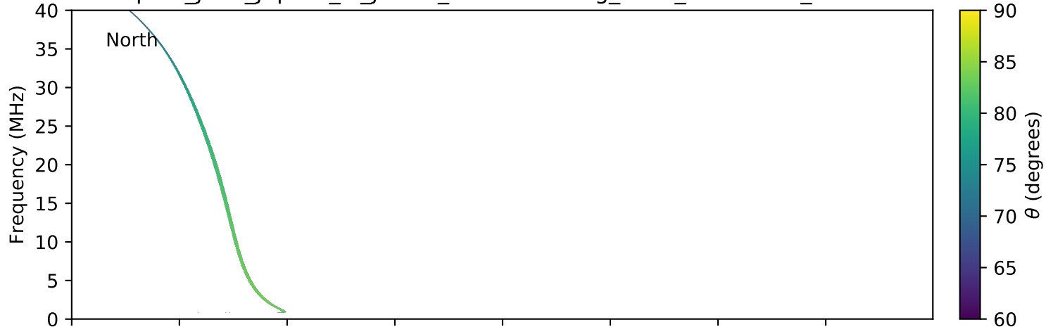
expres_juno_jupiter_io_jrm09_lossc-wid1deg_3kev_20170916_v01.cdf
