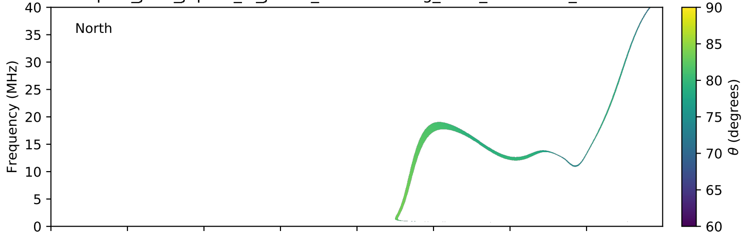
expres_juno_jupiter_io_jrm09_lossc-wid1deg_3kev_20170915_v01.cdf
