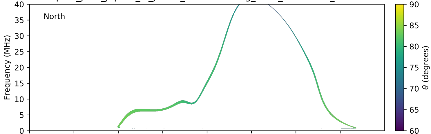
expres_juno_jupiter_io_jrm09_lossc-wid1deg_3kev_20170910_v01.cdf
