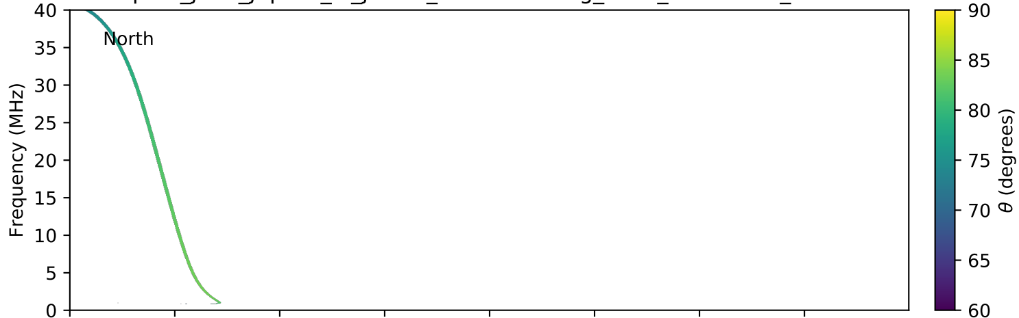
expres_juno_jupiter_io_jrm09_lossc-wid1deg_3kev_20170909_v01.cdf
