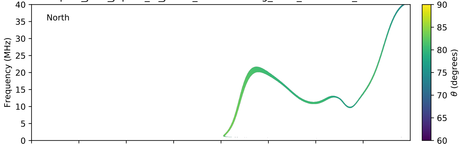
expres_juno_jupiter_io_jrm09_lossc-wid1deg_3kev_20170908_v01.cdf
