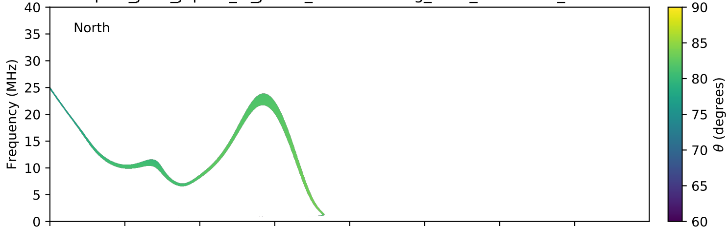
expres_juno_jupiter_io_jrm09_lossc-wid1deg_3kev_20170907_v01.cdf
