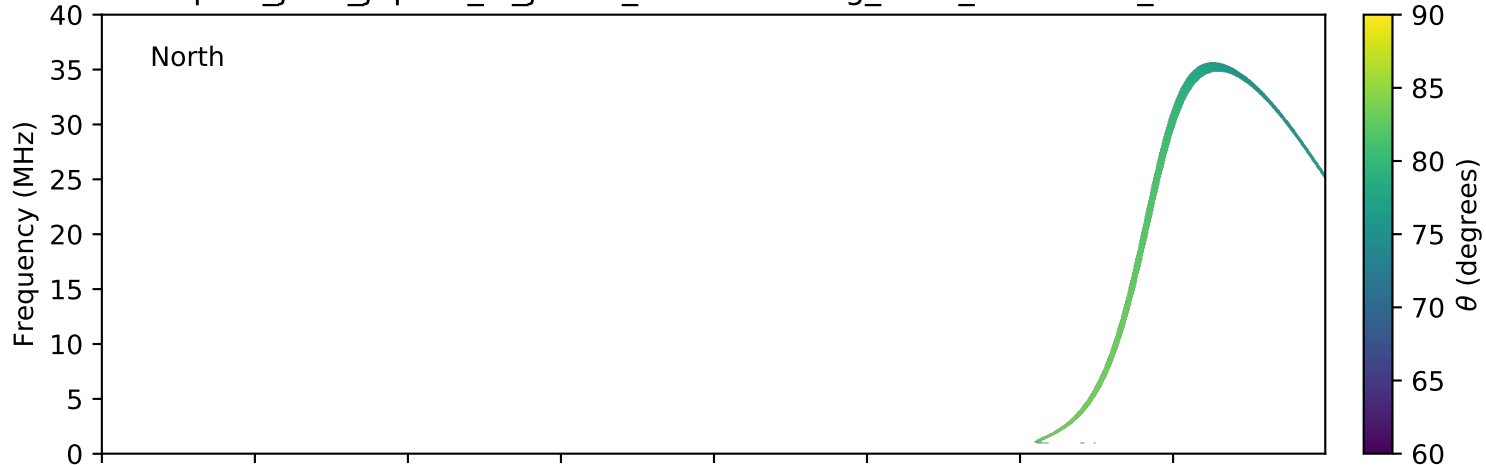
expres_juno_jupiter_io_jrm09_lossc-wid1deg_3kev_20170906_v01.cdf
