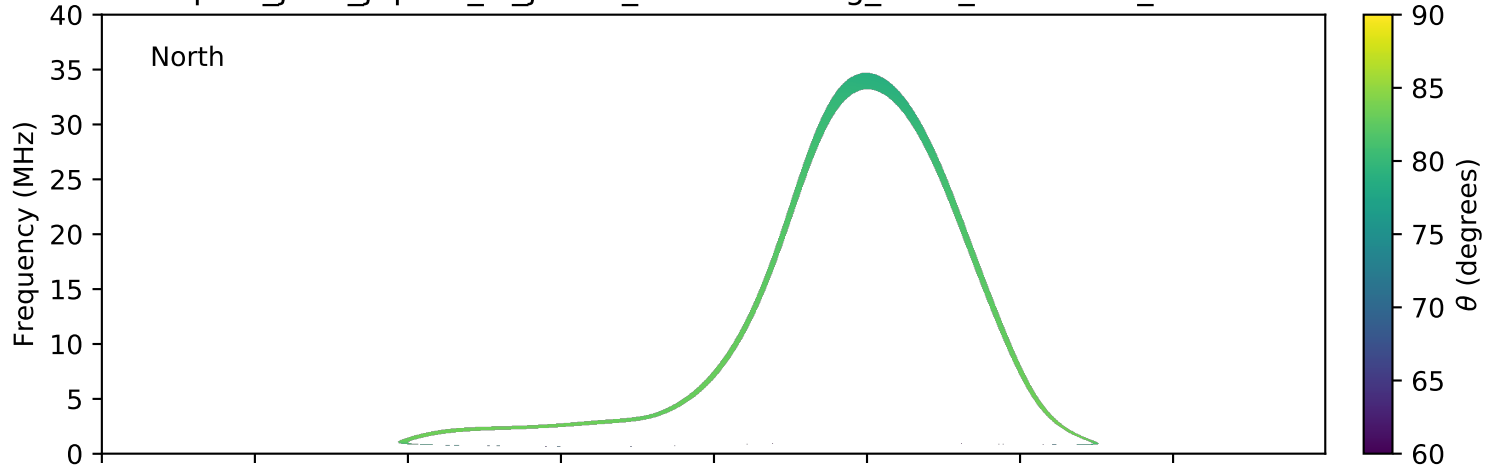
expres_juno_jupiter_io_jrm09_lossc-wid1deg_3kev_20170903_v01.cdf
