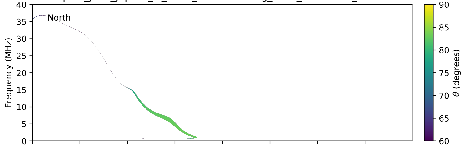
expres_juno_jupiter_io_isaac_lossc-wid1deg_3kev_20170930_v01.cdf
