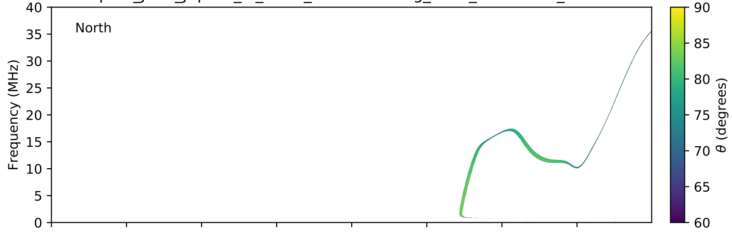
expres_juno_jupiter_io_isaac_lossc-wid1deg_3kev_20170929_v01.cdf
