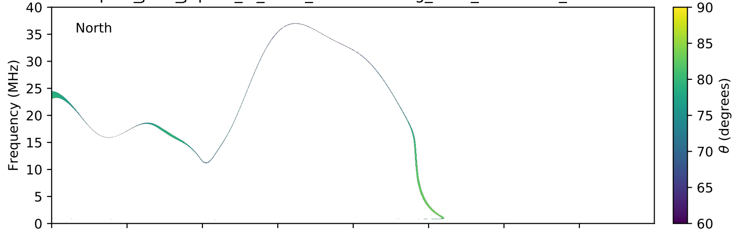
expres_juno_jupiter_io_isaac_lossc-wid1deg_3kev_20170928_v01.cdf
