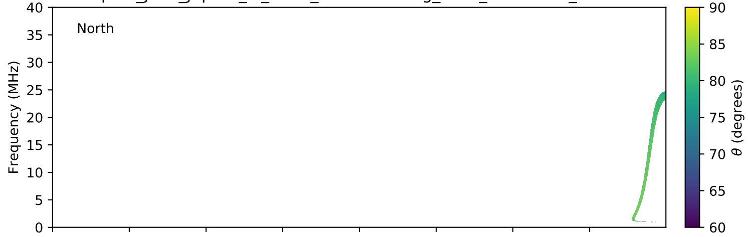
expres_juno_jupiter_io_isaac_lossc-wid1deg_3kev_20170927_v01.cdf
