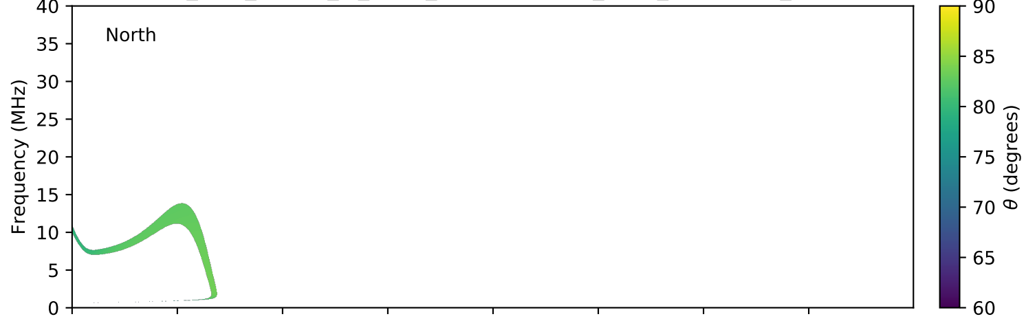
expres_juno_jupiter_io_isaac_lossc-wid1deg_3kev_20170925_v01.cdf
