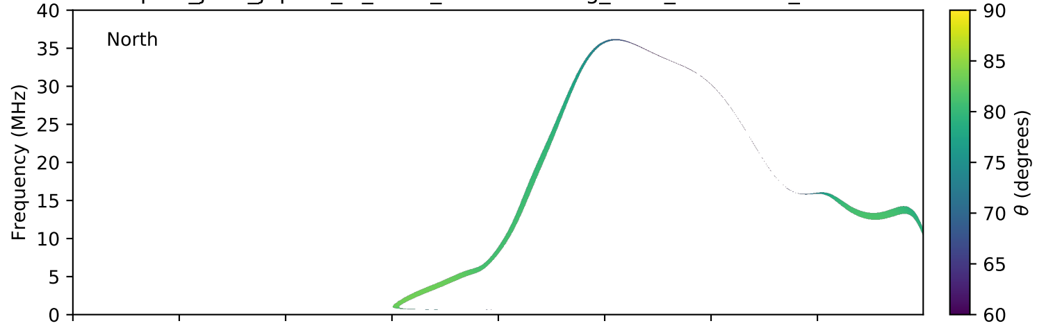
expres_juno_jupiter_io_isaac_lossc-wid1deg_3kev_20170924_v01.cdf
