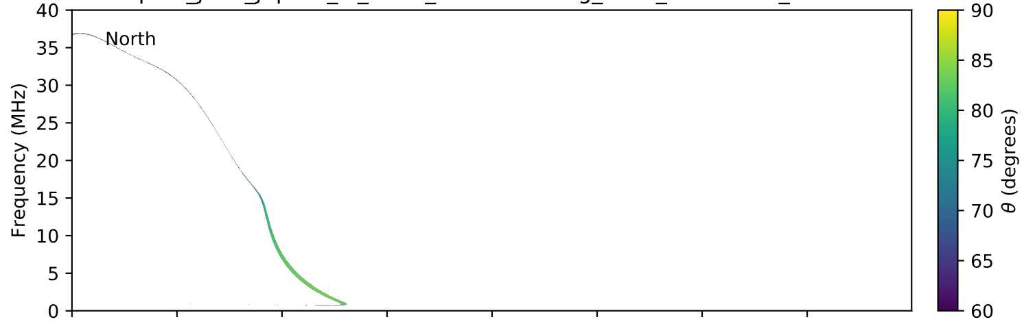
expres_juno_jupiter_io_isaac_lossc-wid1deg_3kev_20170923_v01.cdf
