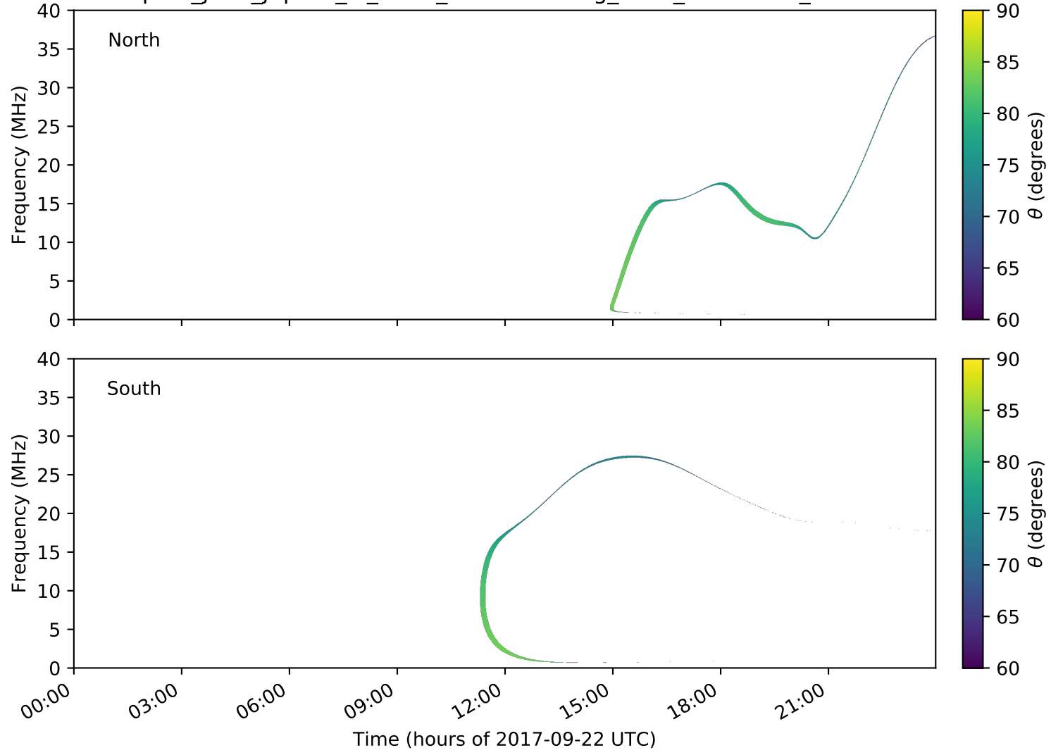
expres_juno_jupiter_io_isaac_lossc-wid1deg_3kev_20170922_v01.cdf
