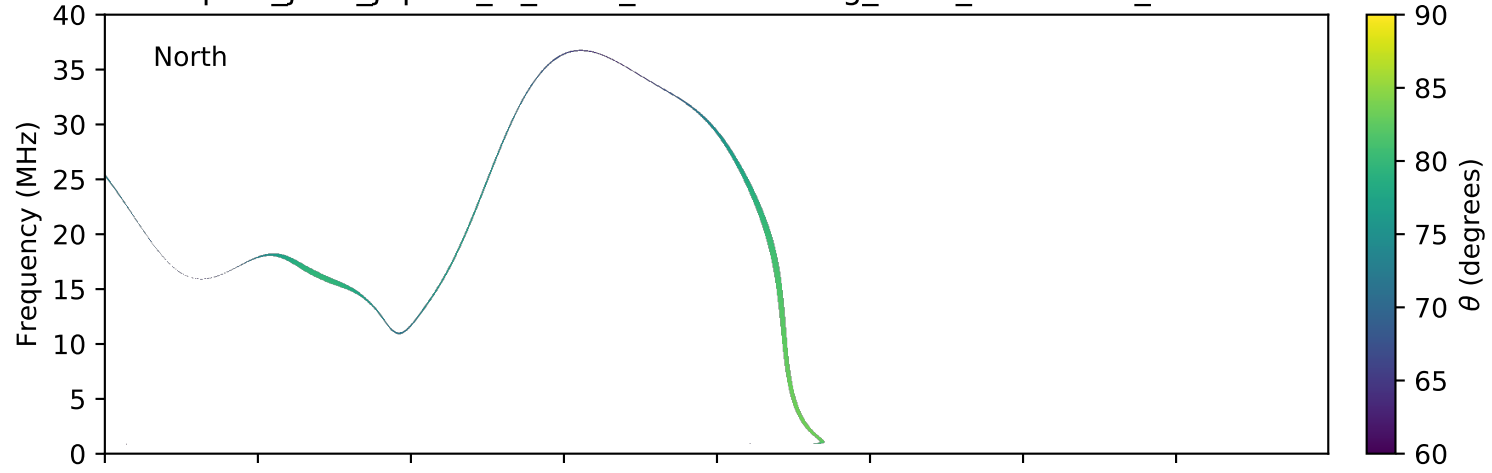
expres_juno_jupiter_io_isaac_lossc-wid1deg_3kev_20170921_v01.cdf
