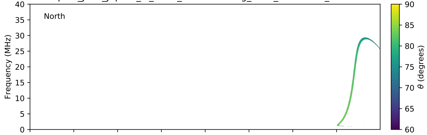
expres_juno_jupiter_io_isaac_lossc-wid1deg_3kev_20170920_v01.cdf
