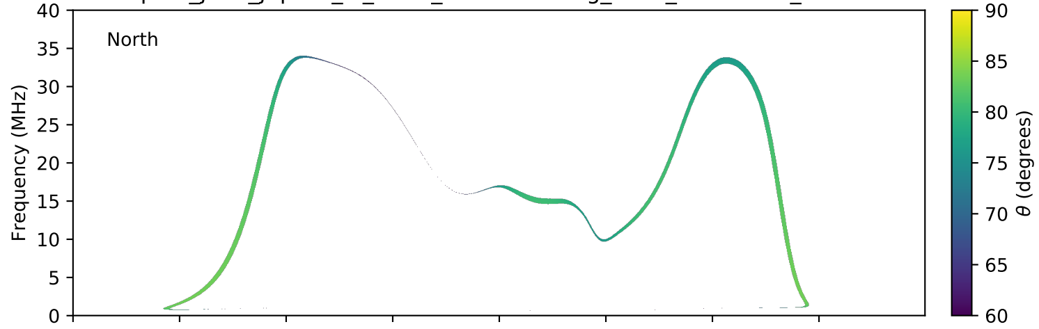
expres_juno_jupiter_io_isaac_lossc-wid1deg_3kev_20170919_v01.cdf
